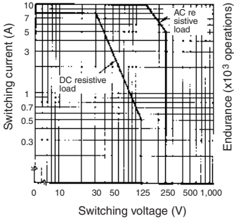
Maximum Switching Power G5LC
