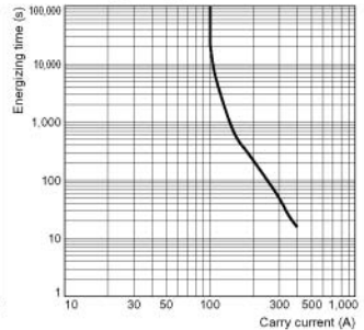
Carry Current vs Energizing Time
