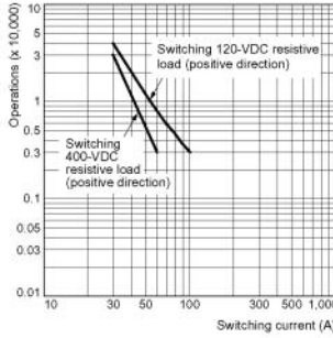
Electrical Endurance (Switching Performance)
