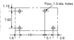
Mounting Holes (Bottom View)
