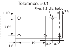
Mounting Holes (Bottom View)
