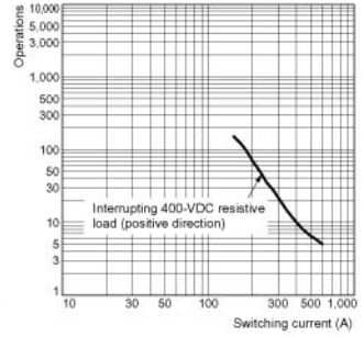
Electrical Endurance (Interruption Performance)
