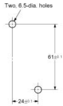
Mounting Hole Dimensions (TOP VIEW)
