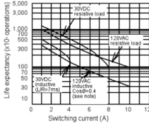
Life Expectancy G5LB-1
