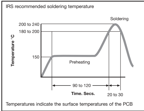
Mounting temperature for Lead solder mounting
