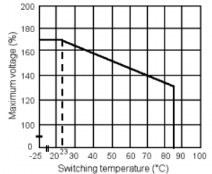
Ambient Temp. Vs Max. Voltage
