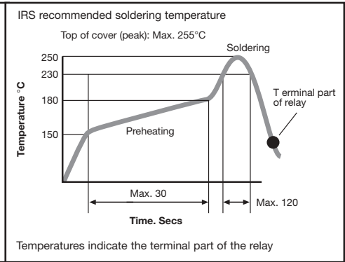
Mounting temperature for Lead-Free solder mounting
