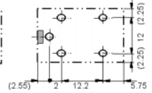
Mounting Holes (Bottom View) Tolerance: \pm 0.1\text{mm}
