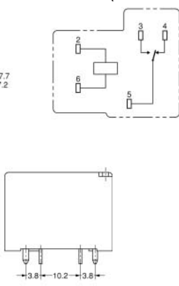
Terminal Arrangement/Internal Connections (Bottom View)
