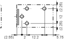
Mounting Holes (Bottom View) Tolerance: \pm 0.1\text{mm}
